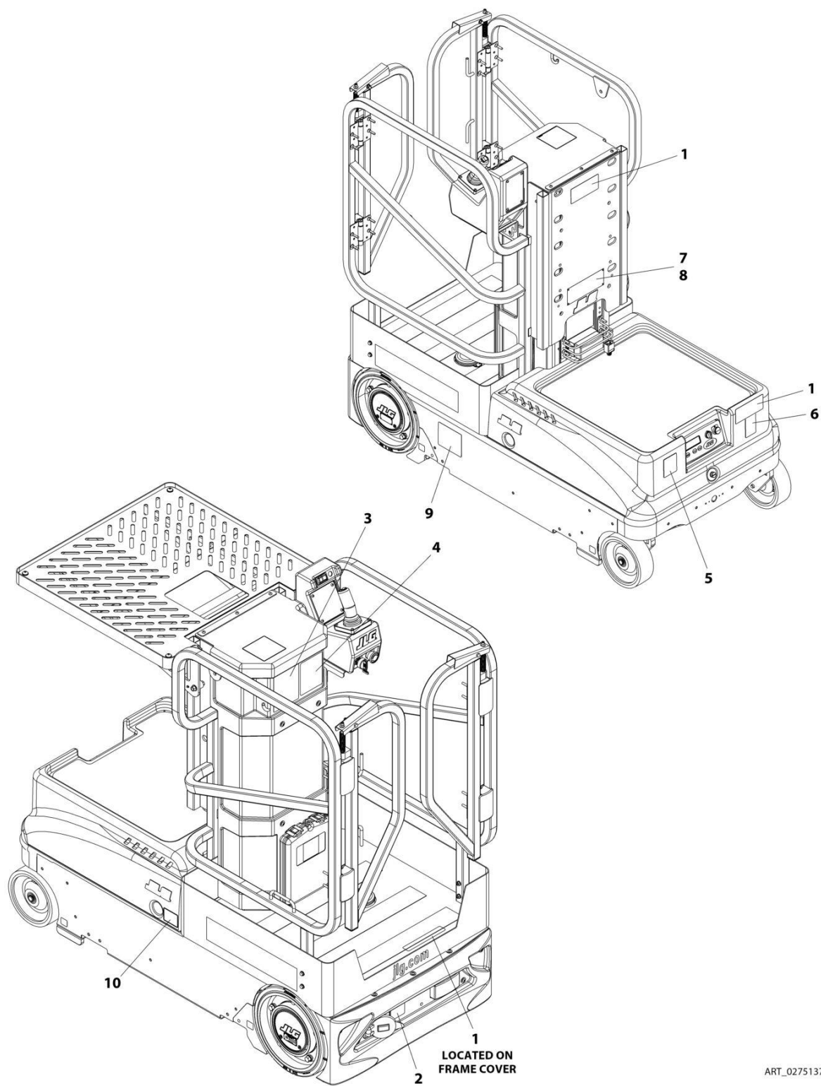
FIGURE 8-17. DECAL INSTALLATION - JAPAN SPECS (JAPANESE LANGUAGE) (MANUAL TRAY)
