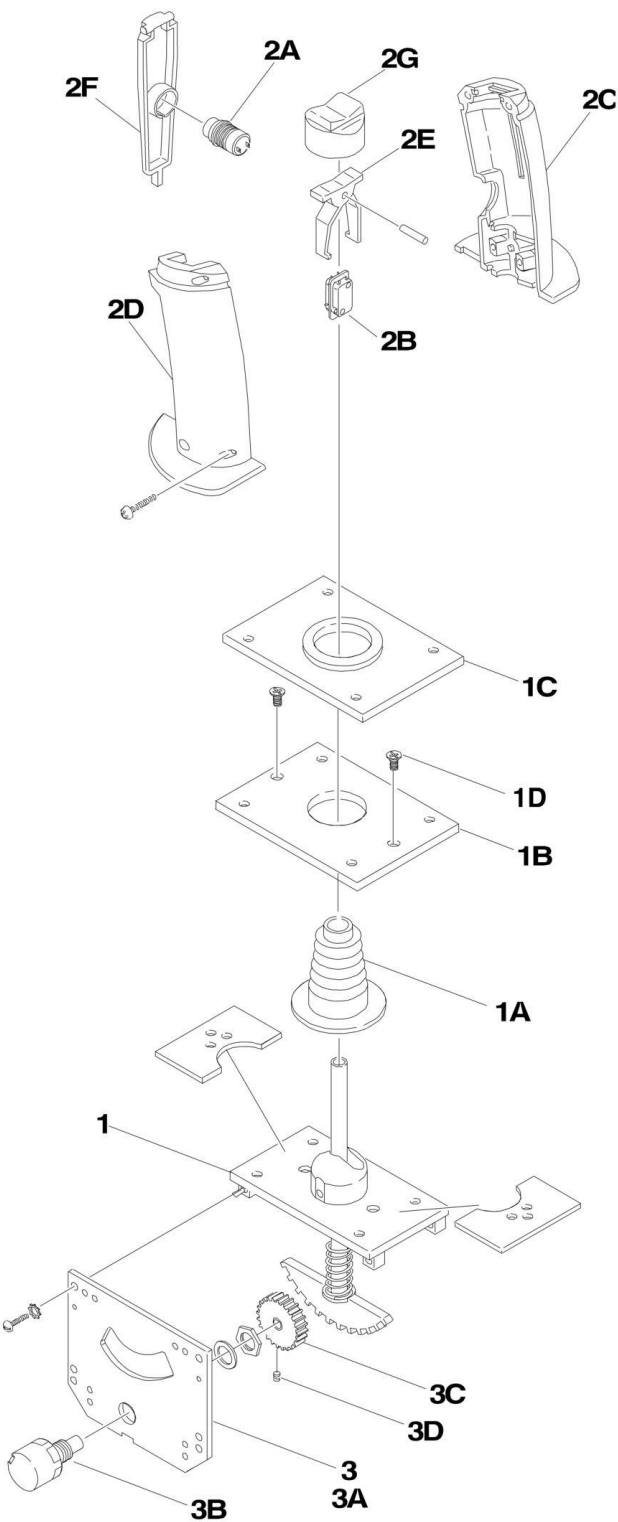
FIGURE 4-6. DRIVE/STEER P/Q CONTROLLER ASSEMBLY (Prior to SN 0200142023)
