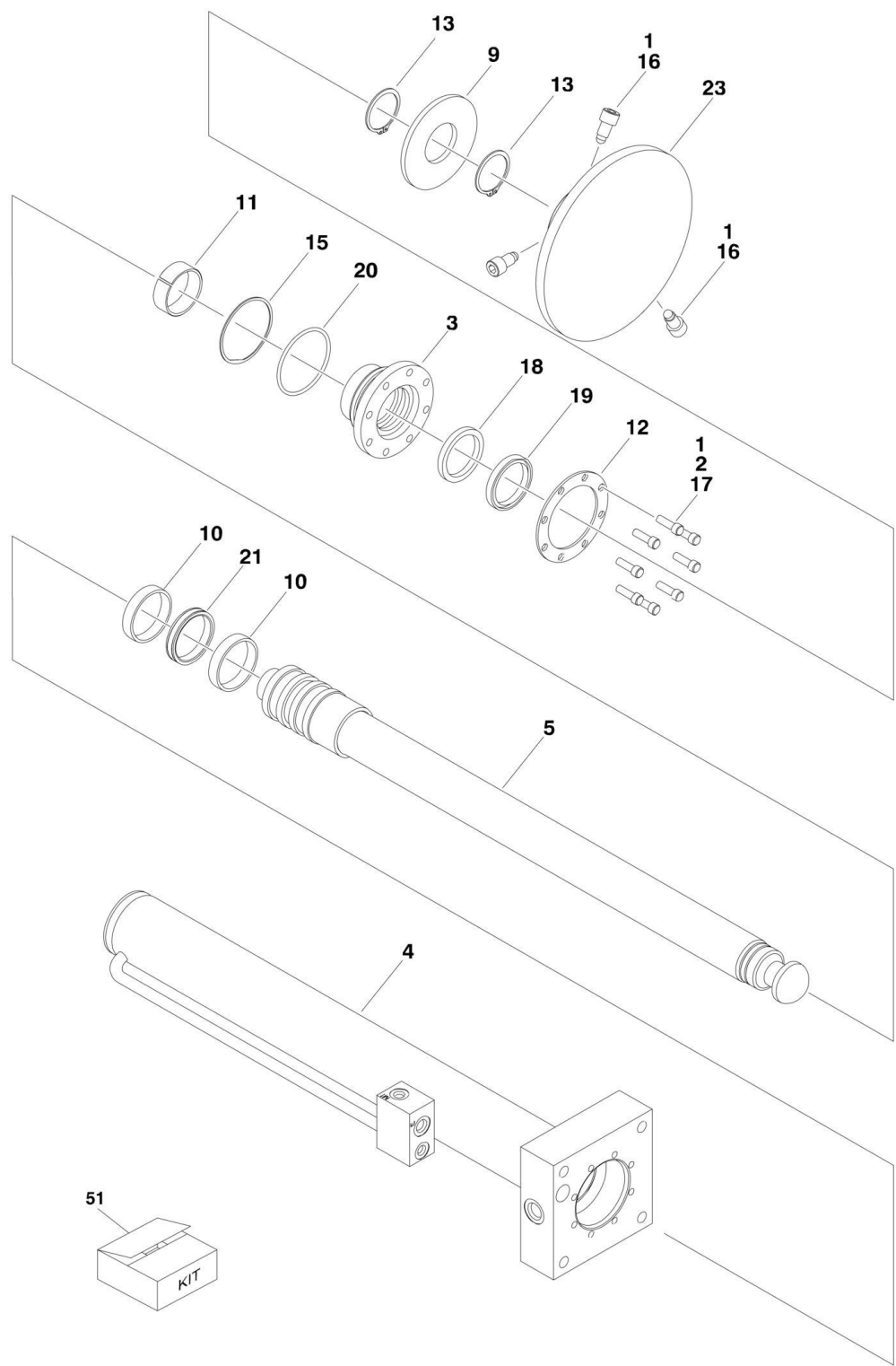
FIGURE 5-3. LEVELING JACKS CYLINDER ASSEMBLY (AUTO LEVEL) (SN 0200141689 through 0200269760)
