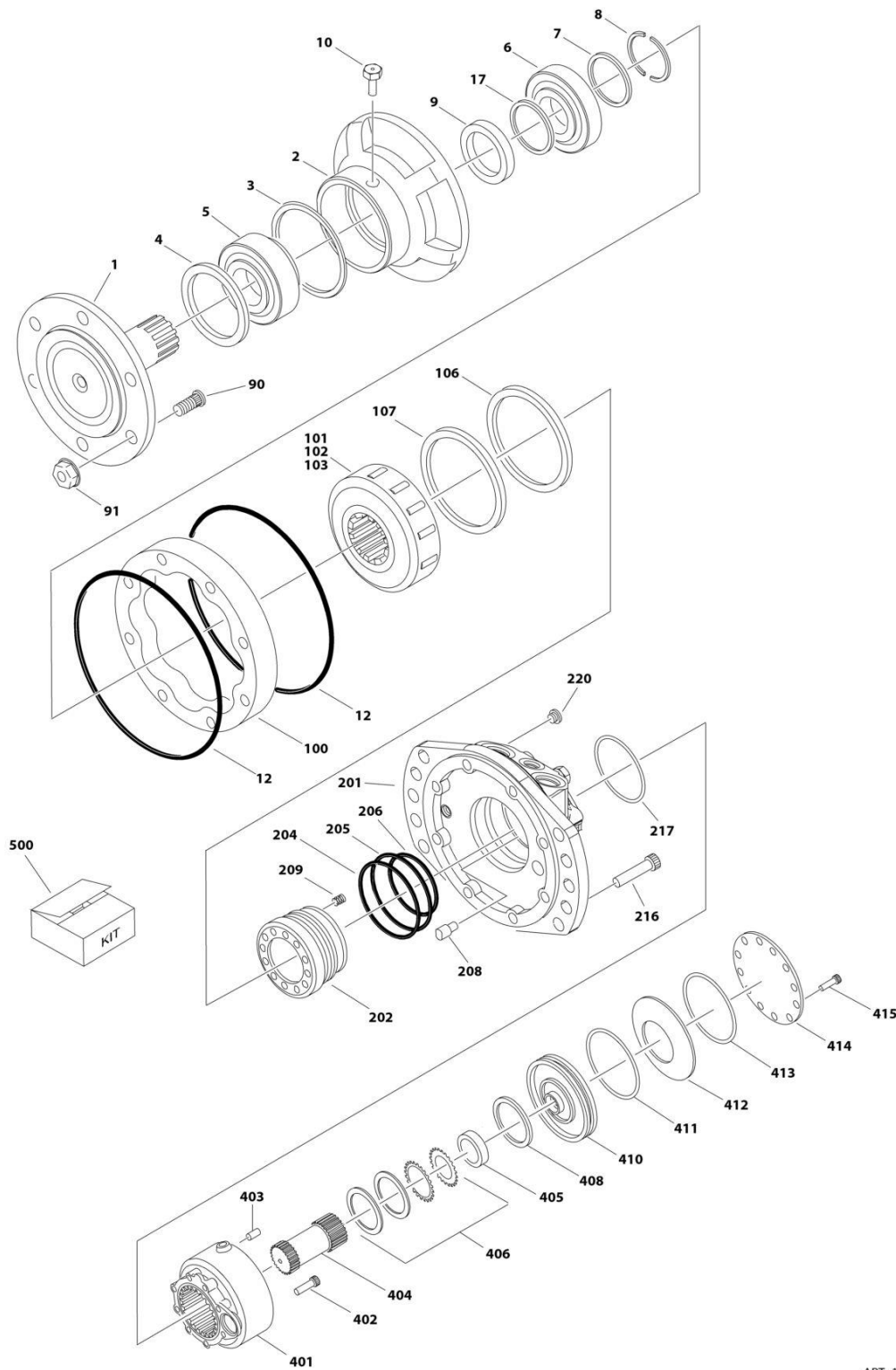
FIGURE 1-4. MOTOR/BRAKE/HUB ASSEMBLY (REAR) (SN 0200268450 through 0200269760)
